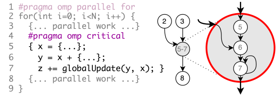
Fig. 3. Capturing properties of a region into hierarchical nodes with traits
