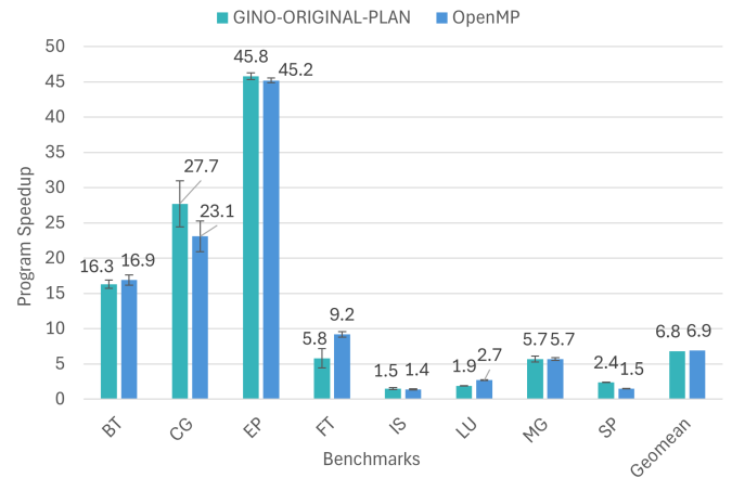
Fig. 12. The speedup on 56 cores with the developers' original parallel execution plans with GINO versus clang OpenMP over 8 NAS benchmarks.
