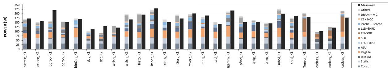
Figure 4.16: AccelWattch validation: AccelWattch SASS SIM modeling a Volta GV100.
