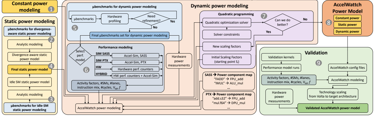
Figure 4.8: AccelWattch power modeling flowchart.
