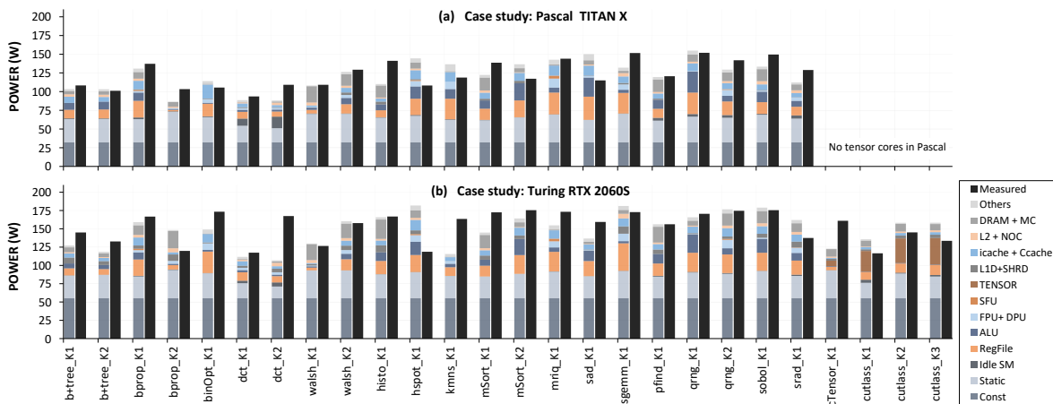
Figure 4.18: Case studies: AccelWattch SASS SIM (tuned for Volta), applied to model Pascal and Turing architectures.
